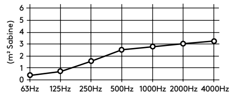
Equivalent Sound Absorption Area (m 2 Sabine)/Unit*
