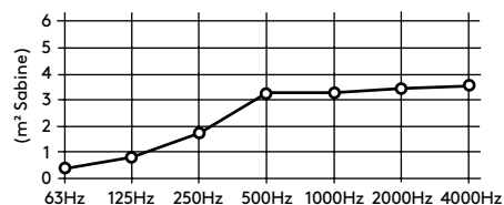
Equivalent Sound Absorption Area (m 2 Sabine)/Unit*
