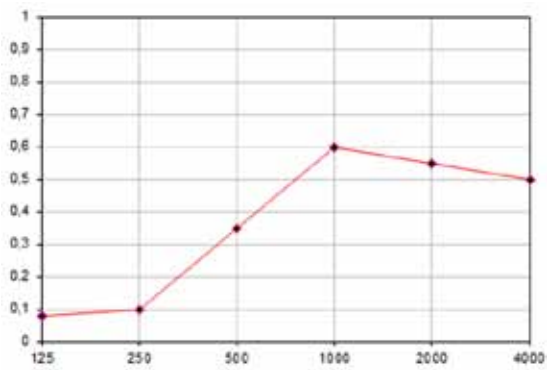
SOUND ABSORPTION MULTIMIX
