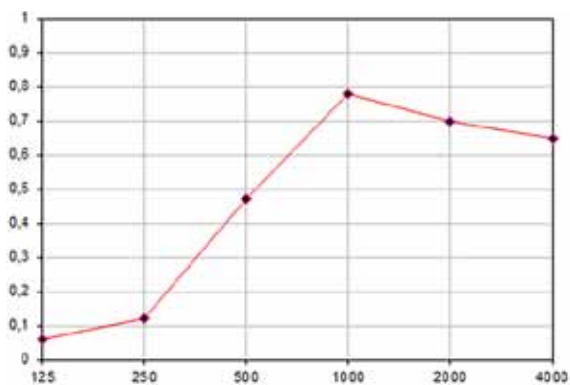
SOUND ABSORPTION ALP
