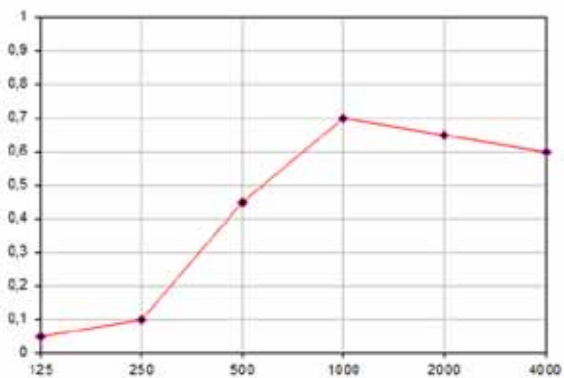
SOUND ABSORPTION TEMA 15 mm, SS-EN ISO 354 and 11654
