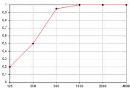
SOUND ABSORPTION LIMBUS
